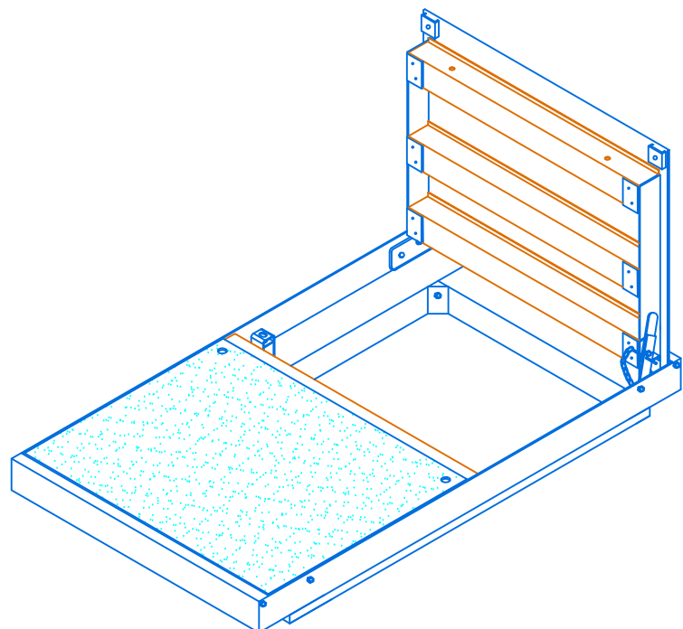
ISOMETRIC DETAIL
