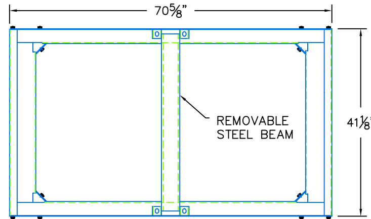
FRAME - PLAN VIEW
