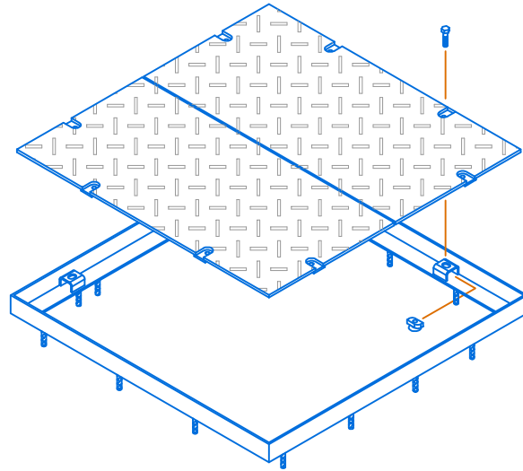
ISOMETRIC DETAIL
