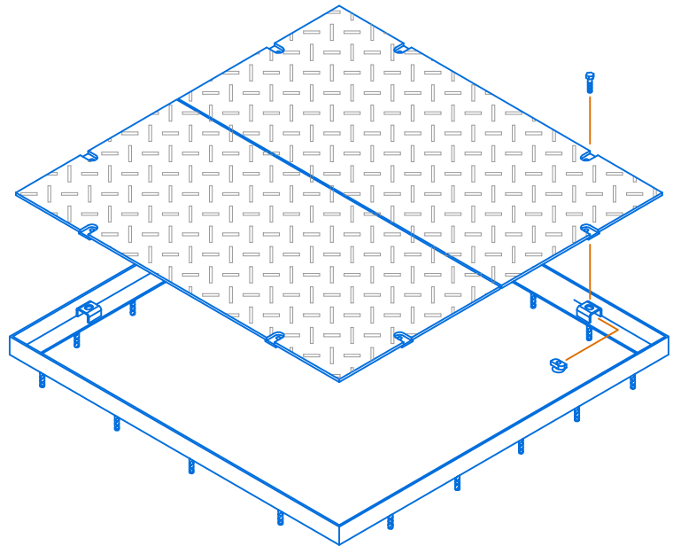
ISOMETRIC DETAIL
