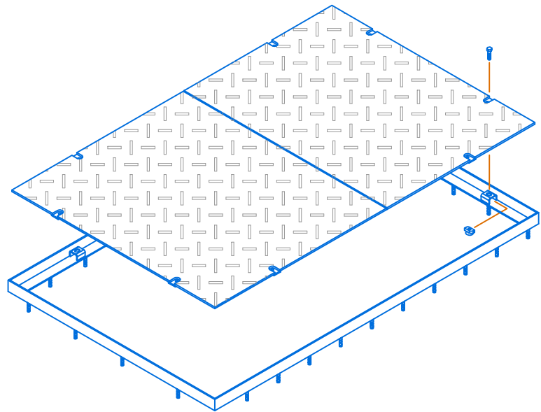
ISOMETRIC DETAIL
