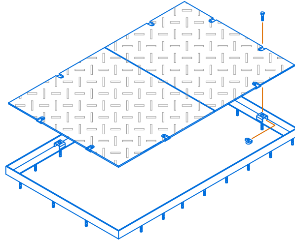
ISOMETRIC DETAIL
